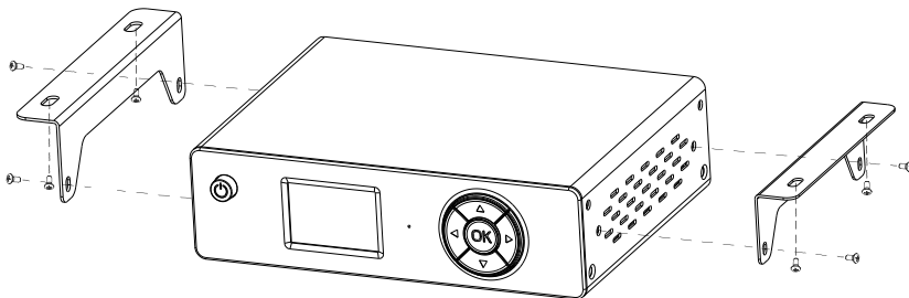
Figure 14.2: Installation of ACU
