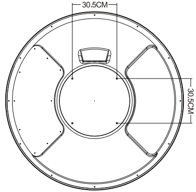
Figure 9: Mounting Hole Position of KM-X8
