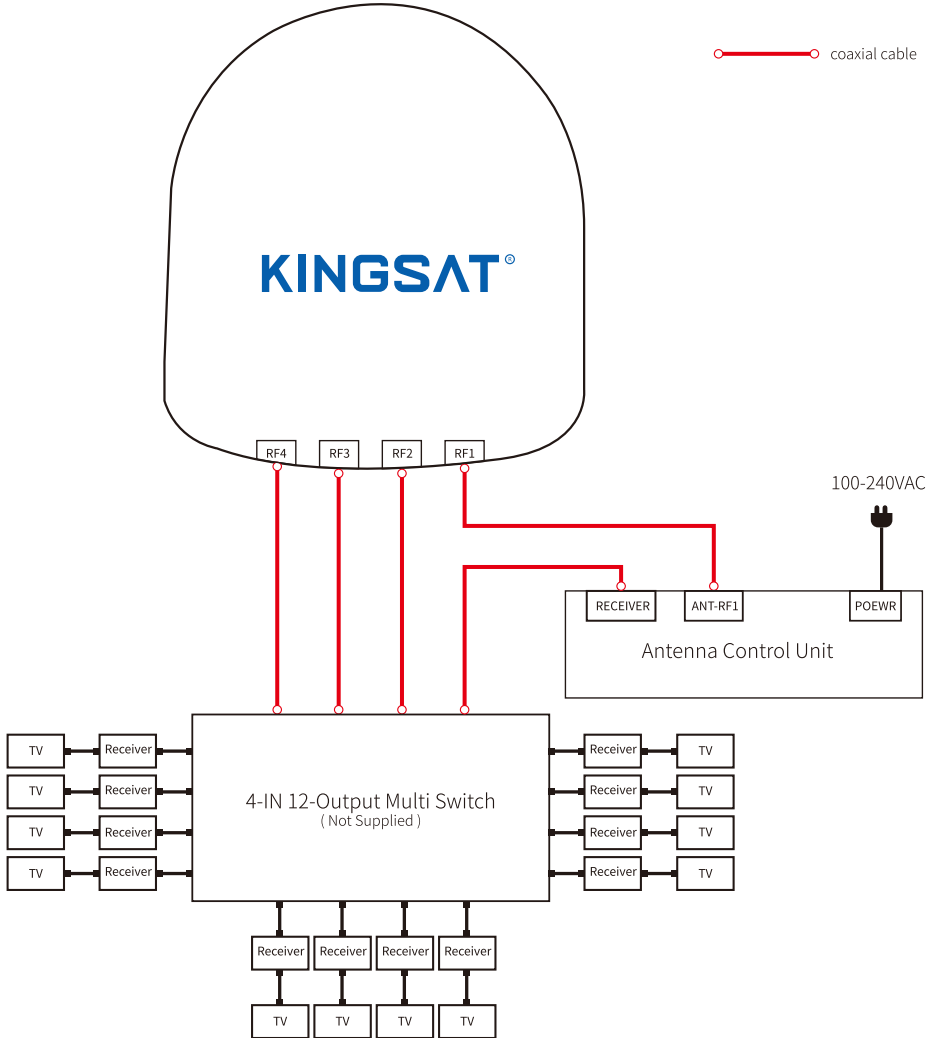
Figure 16: Multi-Receivers Solution
