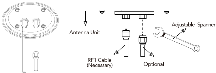
Figure 10: Connectors on Bottom of Antenna
