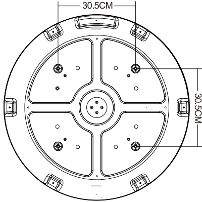
Figure 8: Mounting Hole Position of KM-X6
