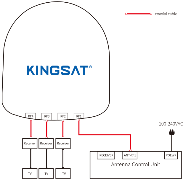
Figure 15: Cable Connection Configuration
