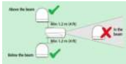
Figure 4: Position of Radar and Antenna
