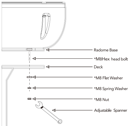
Figure 12 : Mounting the Antenna Model 1
