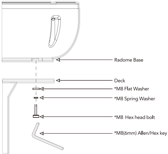
Figure 12 : Mounting the Antenna Model 2
