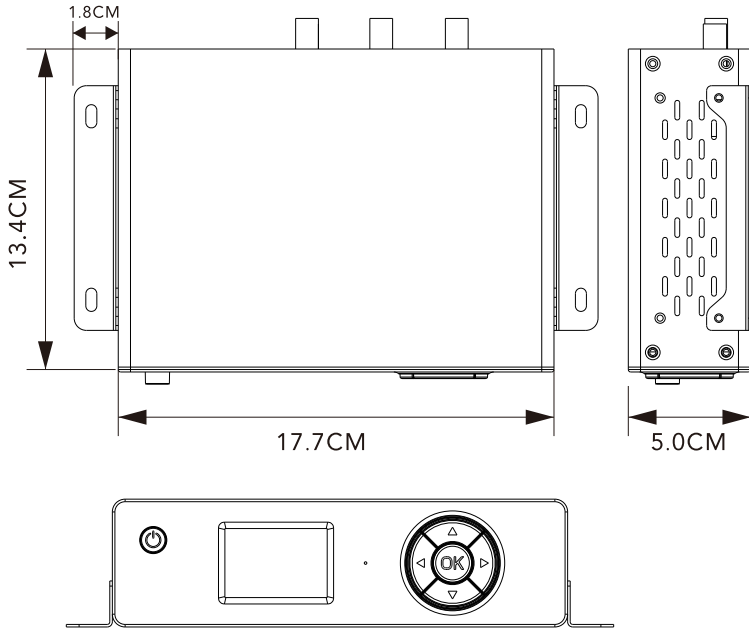
Figure 13: Dimension of ACU
